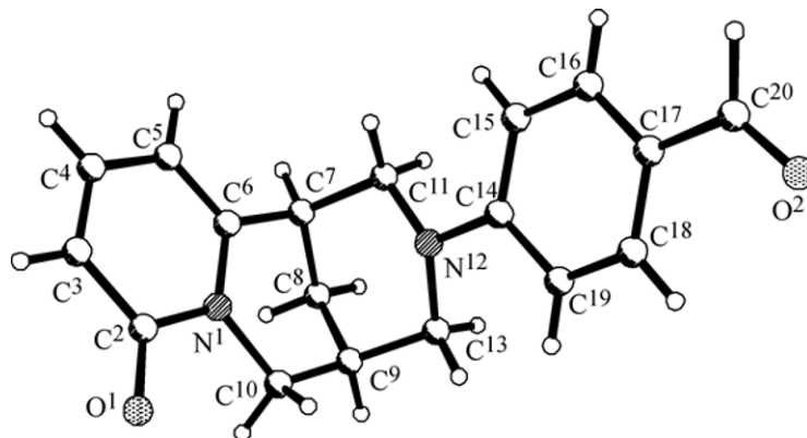
General view of the molecule of 4-( N -cytisinyl)benzaldehyde III .
